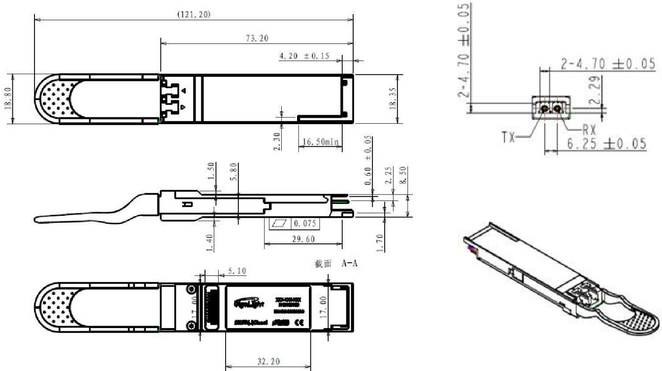
Figure10. Mechanical Specifications
